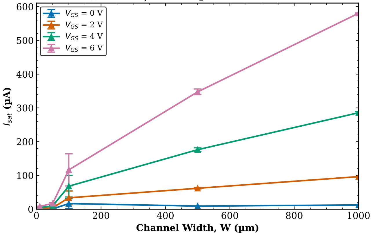
TFT1 Combined (Tr. 1 & 2) I_{sat} vs W | L = 10\text{ }\mu\text{m} (mean \pm std)
